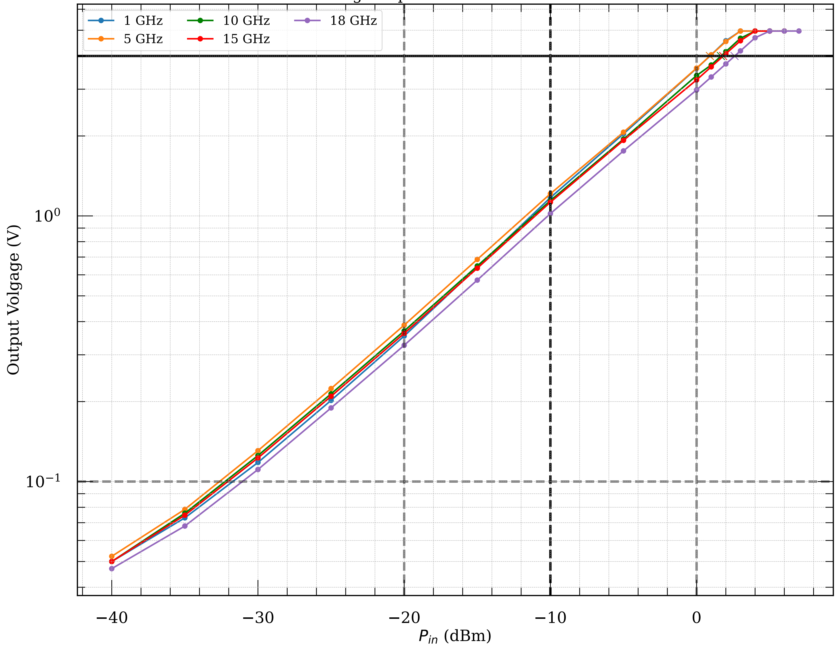
Measured voltage-to-power curve of detector module042
